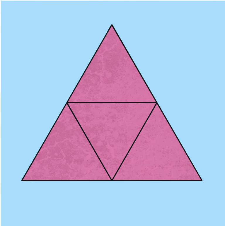
Triangular Pyramid
