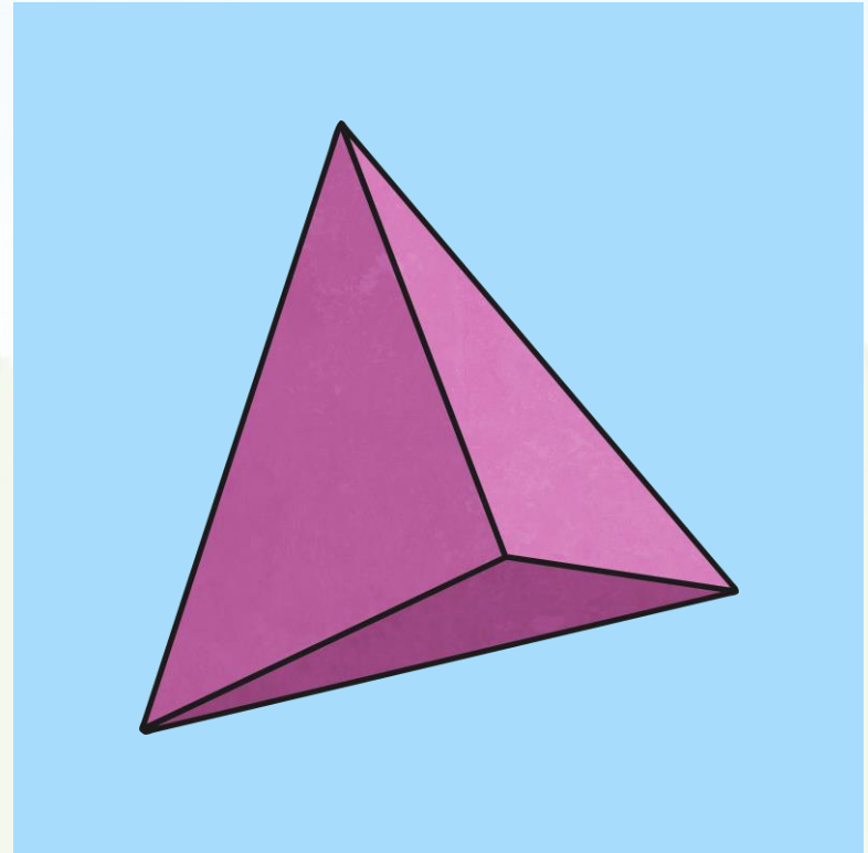
Triangular Pyramid
